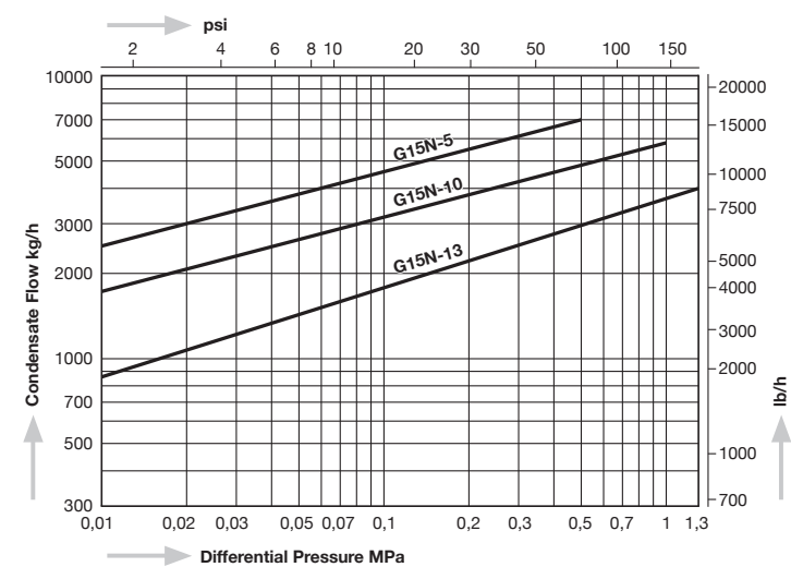
Capacity Chart G15N
